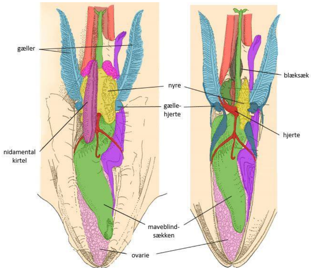
Figur 4.11: Loligos anatomi
